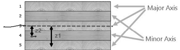
Figure 6 Cross-section of a 5-layer CLT panel
