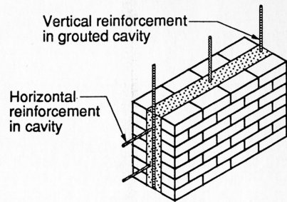
(b) Reinforcement in Cavity
